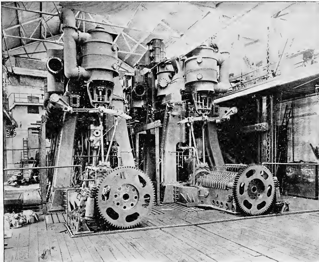
QUADRUPLE-EXPANSION ENGINES OF STEAMER ST. LOUIS.—Built by Wm. Cramp & Sons.
